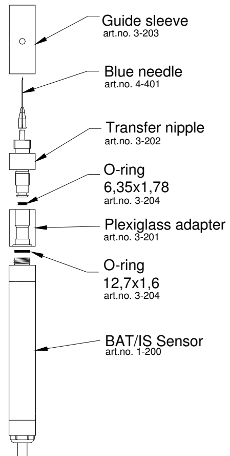
Figure 1a. The BAT/IS-sensor and its components.
