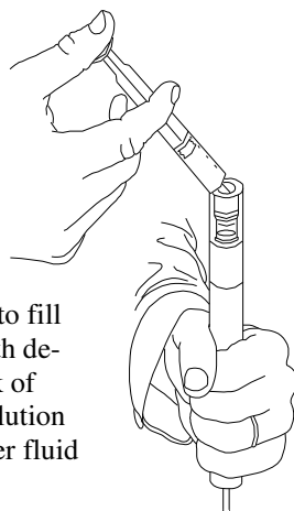
Figure 1c. Bleed the transfer fluid by gently tightening the transfer nipple. Make sure that the O-ring seals inside the plexiglass adapter.
