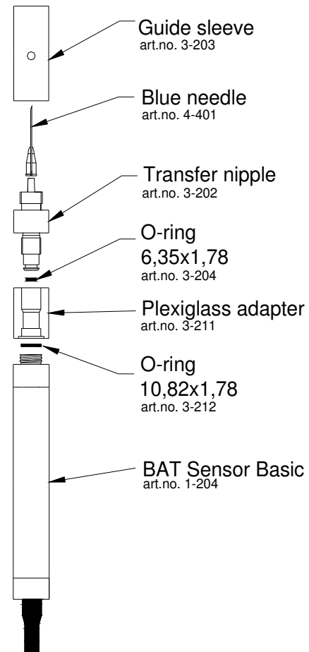
Figure 1a. The BAT-sensor Basic and its components.
